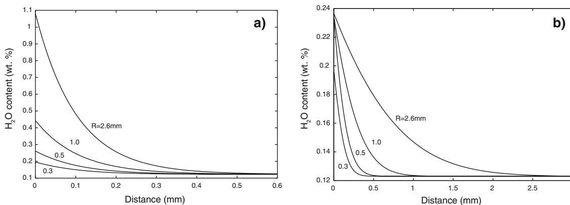
Fig. 5 Model calculations showing the evolution of water concentration away from spherulite boundaries assuming two different spherulite growth laws. Note the different scales for the x- and y-axes. The linear growth law (5a) leads to narrow profiles with a progressive
