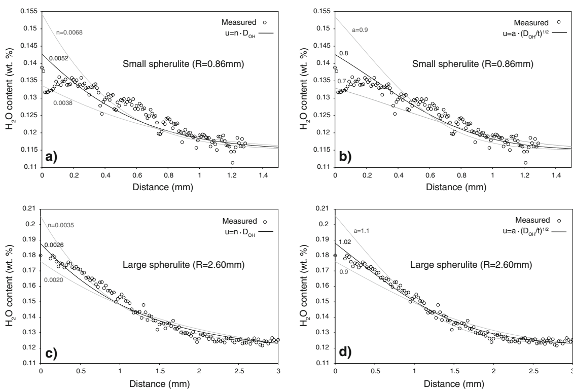
Fig. 6 Comparison between measured water concentration profiles and model calculations. a and c show results for two different spherulites using a linear growth law (i.e., u \sim D_{OH} \cdot t ). b and d show results for two different spherulites using a diffusion-controlled
